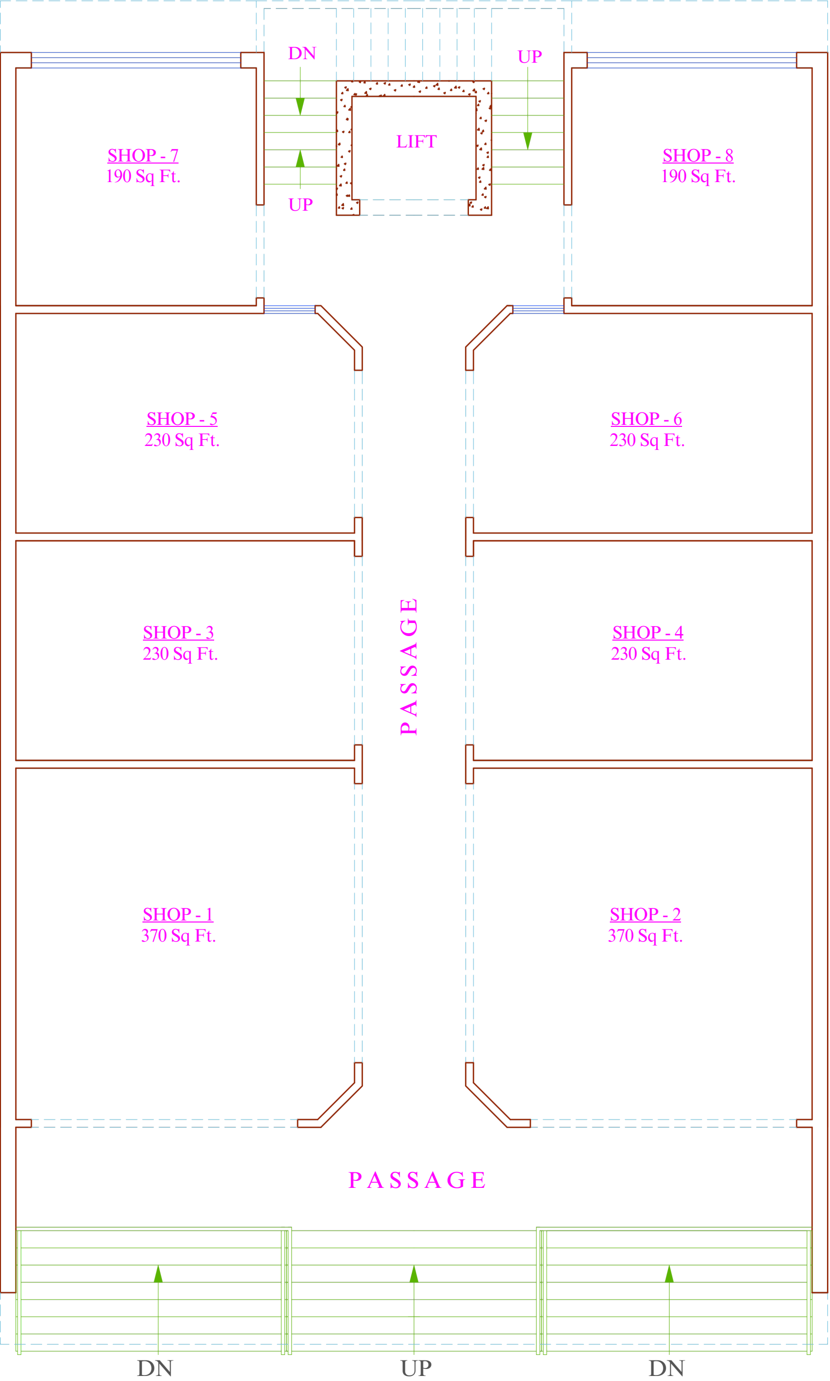
SHOPS - GROUND FLOOR PLAN
